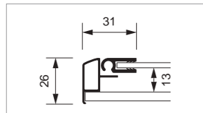
Profiles PX
