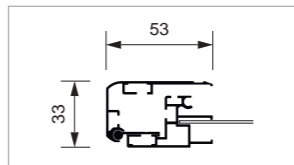
Profiles T
