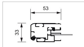
Profiles SCEOS
