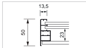
Profiles SCA
